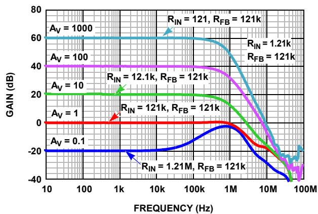
FIGURE 20. CLOSED LOOP GAIN ( R_{FB} = 121k ) vs FREQUENCY
