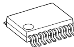
SSOP18-P-225-0.65
