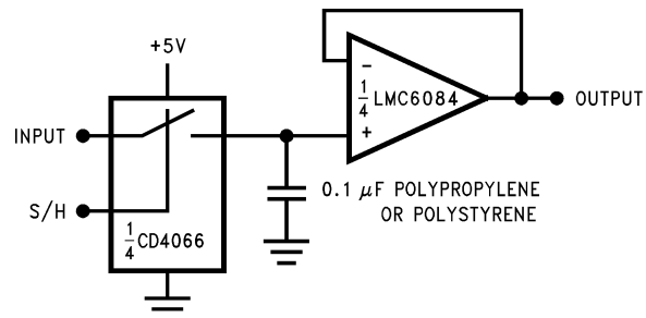
FIGURE 8. Low-Leakage Sample and Hold
