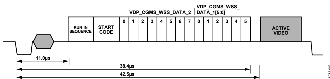
Figure 42. WSS Waveform
