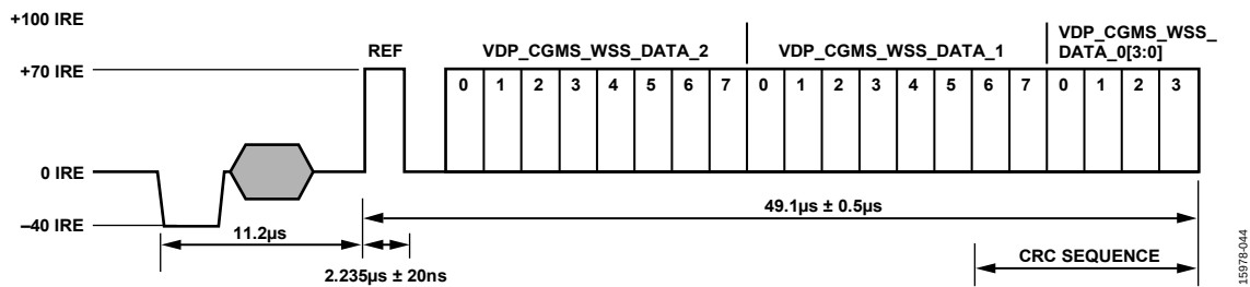
Figure 43. CGMS Waveform
