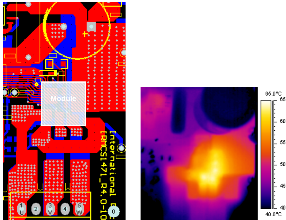
Figure 7: PCB layout example and corresponding thermal image (6kHz, 2P, 2oz, \Delta T_{\text{ca}}=40^\circ\text{C} , V_+ = 150\text{V} , I_u = 427\text{mA} , P_o = 94\text{W} )
