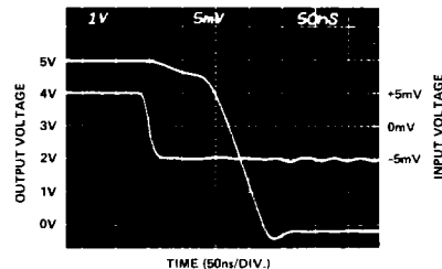
COMPARATOR OUTPUT RESPONSE TIME (2kΩ PULL-UP RESISTOR, T_A = 25^\circ\text{C} )
