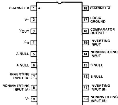
18-PIN HERMETIC DIP (X-Suffix) EPOXY DIP (P-Suffix)
