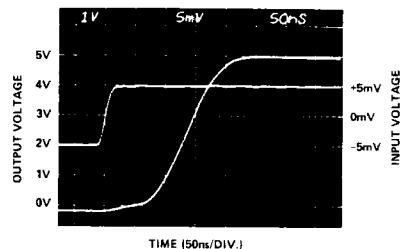
COMPARATOR OUTPUT RESPONSE TIME (2k \Omega PULL-UP RESISTOR, T_A = 25^\circ C )
