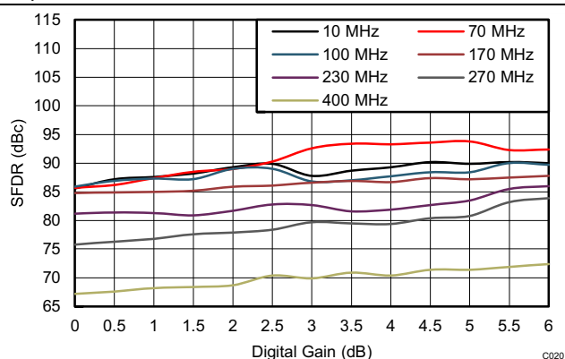
Figure 20. SFDR vs Digital Gain and Input Frequency
