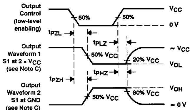
VOLTAGE WAVEFORMS
