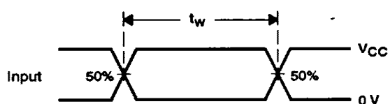
VOLTAGE WAVEFORMS
