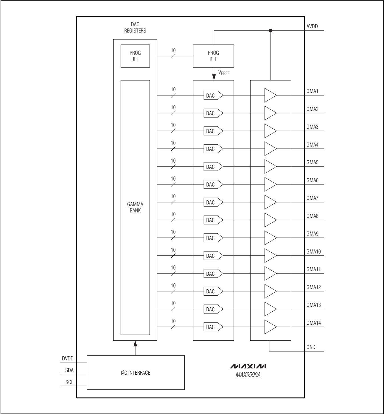
Functional Diagram
