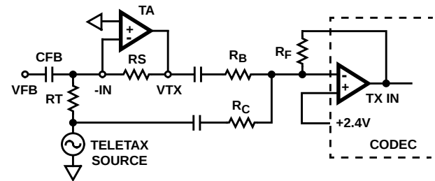
FIGURE 21. TELETAX SIGNALLING
