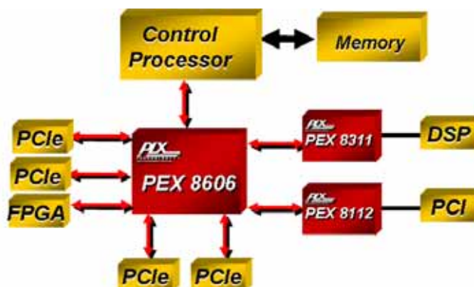
Figure 2-2. Fan-In/Fan-Out Usage
