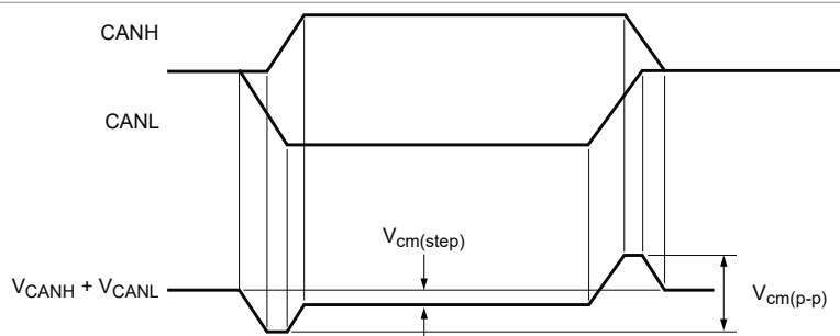
Figure 7. CAN bus common-mode voltage
