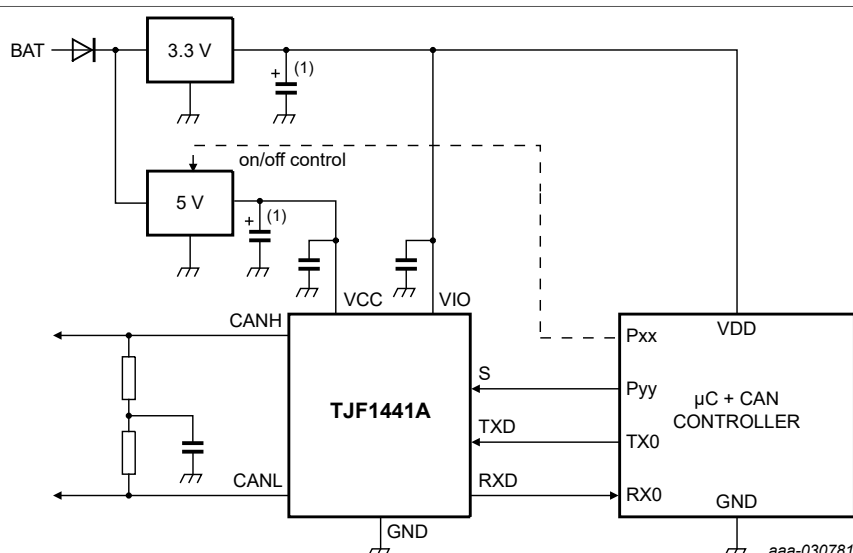
Figure 8. Typical application
