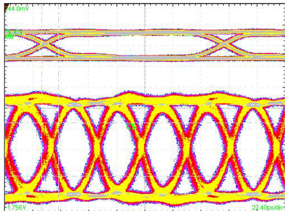
Eye Diagram @ 28 Gbps
