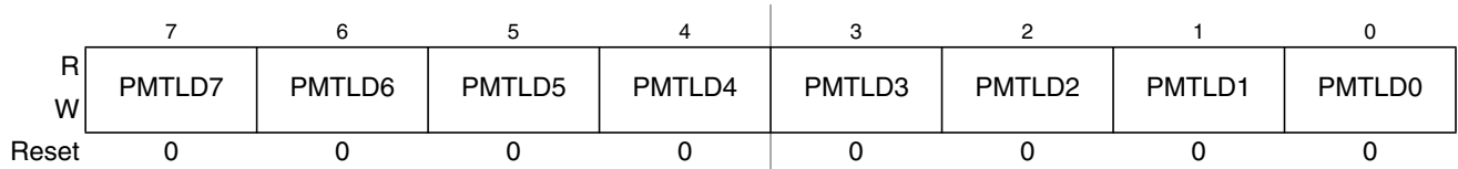
Figure 18-10. PIT Micro Timer Load Register 1 (PITMTLD1)
