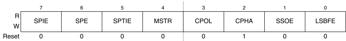
Figure 21-3. SPI Control Register 1 (SPICR1)
