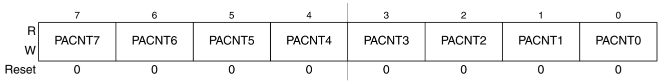
Figure 14-40. Pulse Accumulators Count Register 0 (PACN0)
