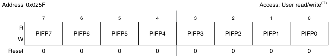
Figure 2-50. Port P Interrupt Flag Register (PIFP)
