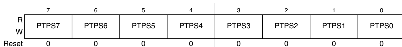
Figure 14-48. Precision Timer Prescaler Select Register (PTPSR)
