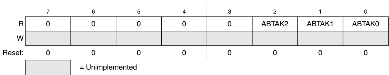
Figure 16-13. MSCAN Transmitter Message Abort Acknowledge Register (CANTAANK)
