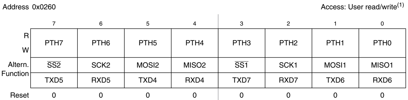
Figure 2-51. Port H Data Register (PTH)
