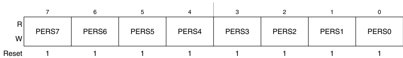
Figure 2-31. Port S Pull Device Enable Register (PERS)
