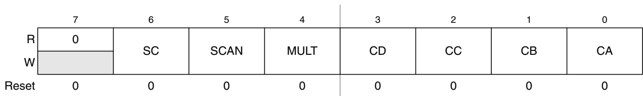
Figure 13-8. ATD Control Register 5 (ATDCTL5)
