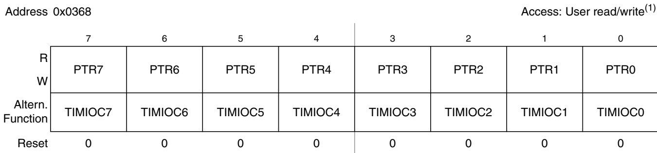
Figure 2-83. Port R Data Register (PTR)
