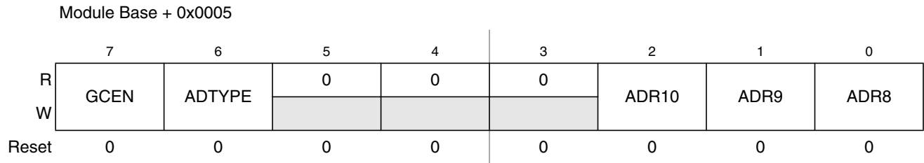
Figure 15-9. IIC Bus Control Register 2(IBCR2)
