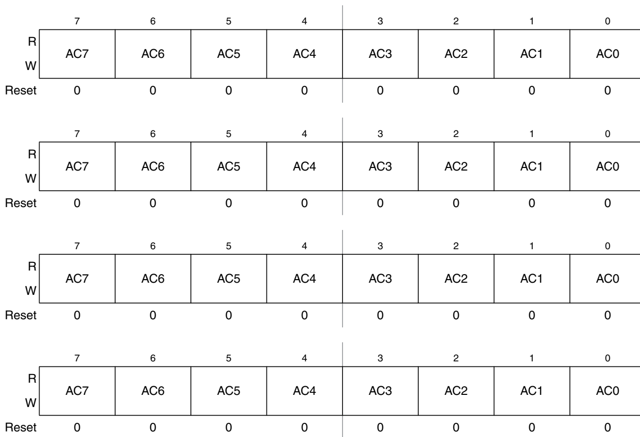
Figure 16-21. MSCAN Identifier Acceptance Registers (Second Bank) — CANIDAR4–CANIDAR7
