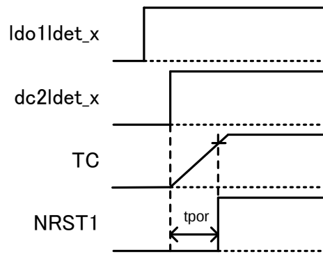
Fig.7.3 Power-on reset
