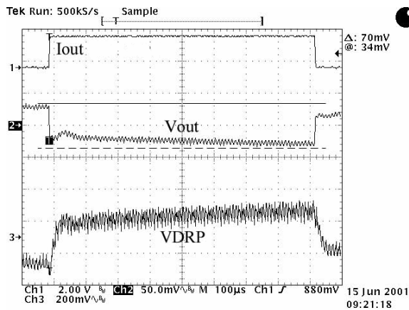
Figure 19. V_{DRP} Tuning Waveforms. The RC Time Constant of the Current Sense Network Is Too Long (Slow): V_{DRP} and V_{OUT} Respond Too Slowly.
