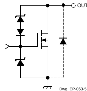
DMOS POWER DRIVER OUTPUT
