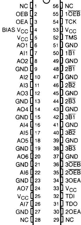
SN54FB2041 . . . WD PACKAGE (TOP VIEW)
