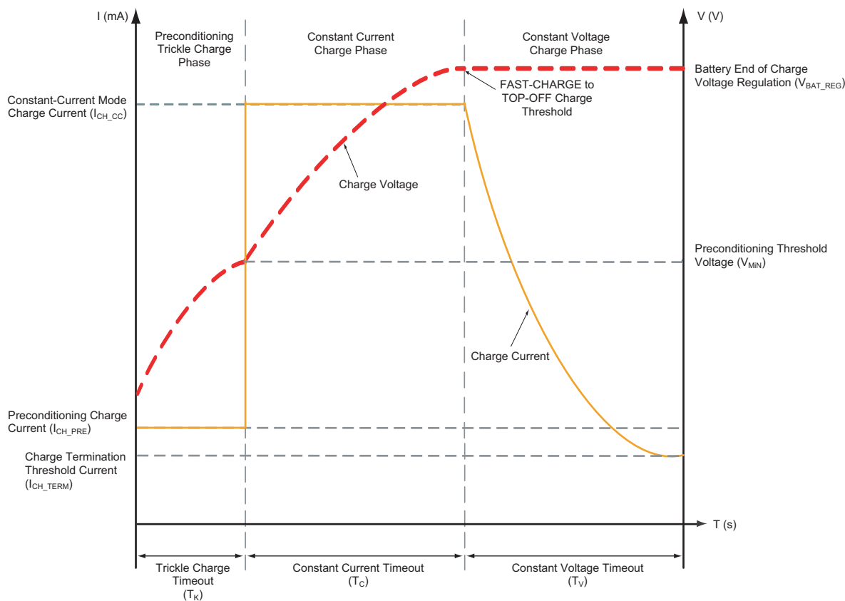
Figure 4: Current vs. Voltage and Charger Time Profile.
