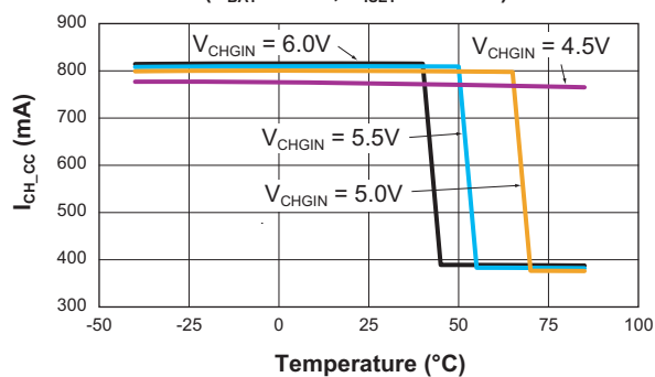
Constant Current Mode Charge Current vs. Temperature ( V_{BAT} = 3.6V ; R_{SET} = 1.24k\Omega )
