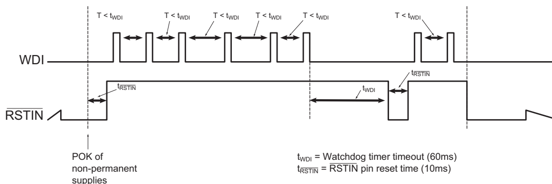
Figure 3: Watchdog Timer Timing Diagram.
