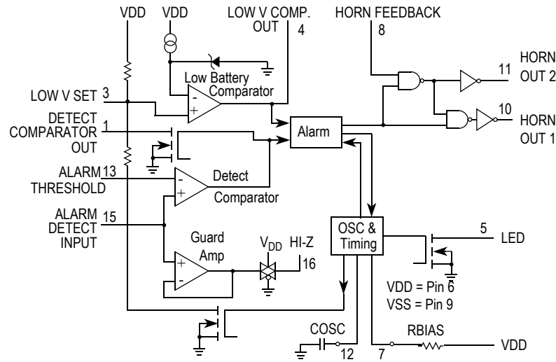
Figure 2. 14600 Block Diagram
