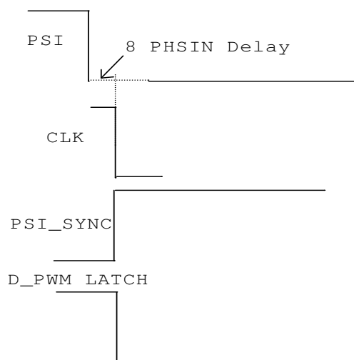
Figure 7: PSI assertion.
