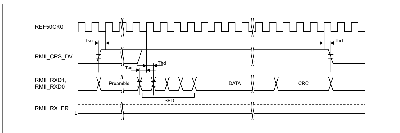
Figure 2.51 RMII reception timing in normal operation
