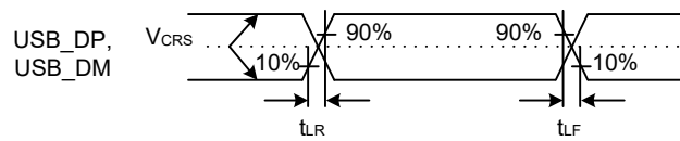
Figure 2.54 USB_DP and USB_DM output timing in low-speed mode
