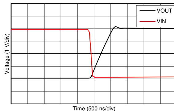
Rising output, 4-V step
