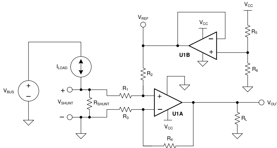
Figure 8-1. Bidirectional Current-Sensing
