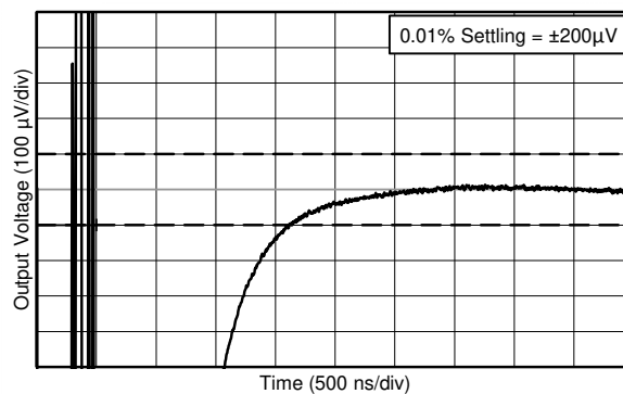
0.01% settling = \pm 200\text{ }\mu\text{V} , 1-V negative step
