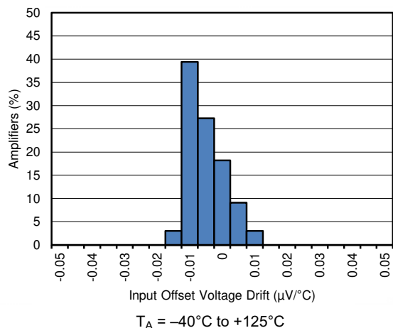
Figure 6-2. Offset Voltage Drift Distribution
