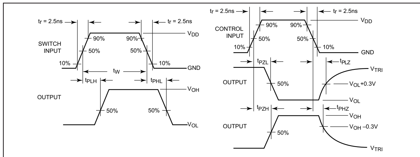
Figure 2. AC Waveforms
