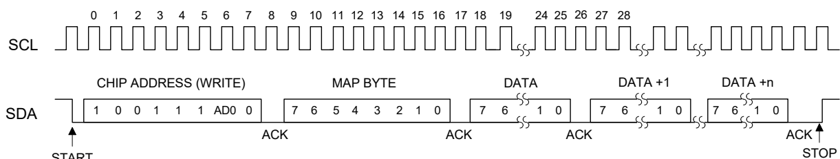
Figure 15. Control Port Timing, I²C Write
