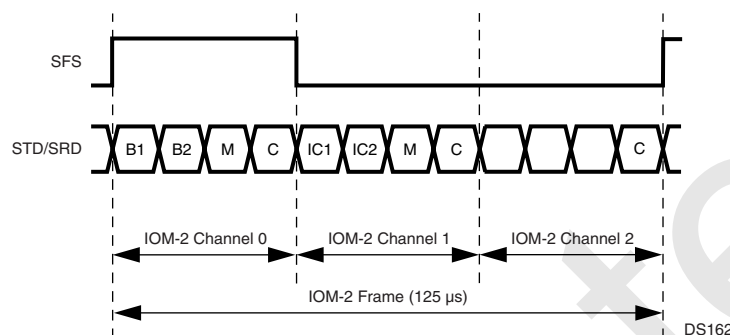
Figure 25. IOM-2 Frame Structure
