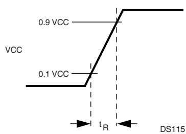
Figure 62. Power-On Reset
