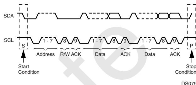
Figure 46. A Complete ACCESS.bus Data Transaction
