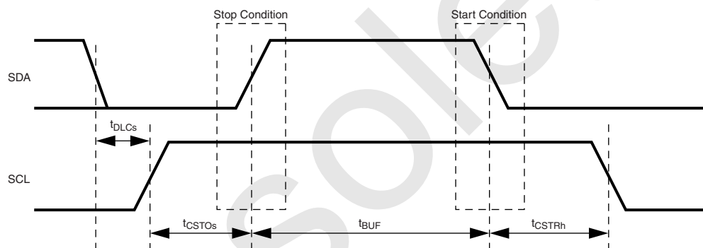
Figure 73. ACB Signals (SDA and SCL) Timing
