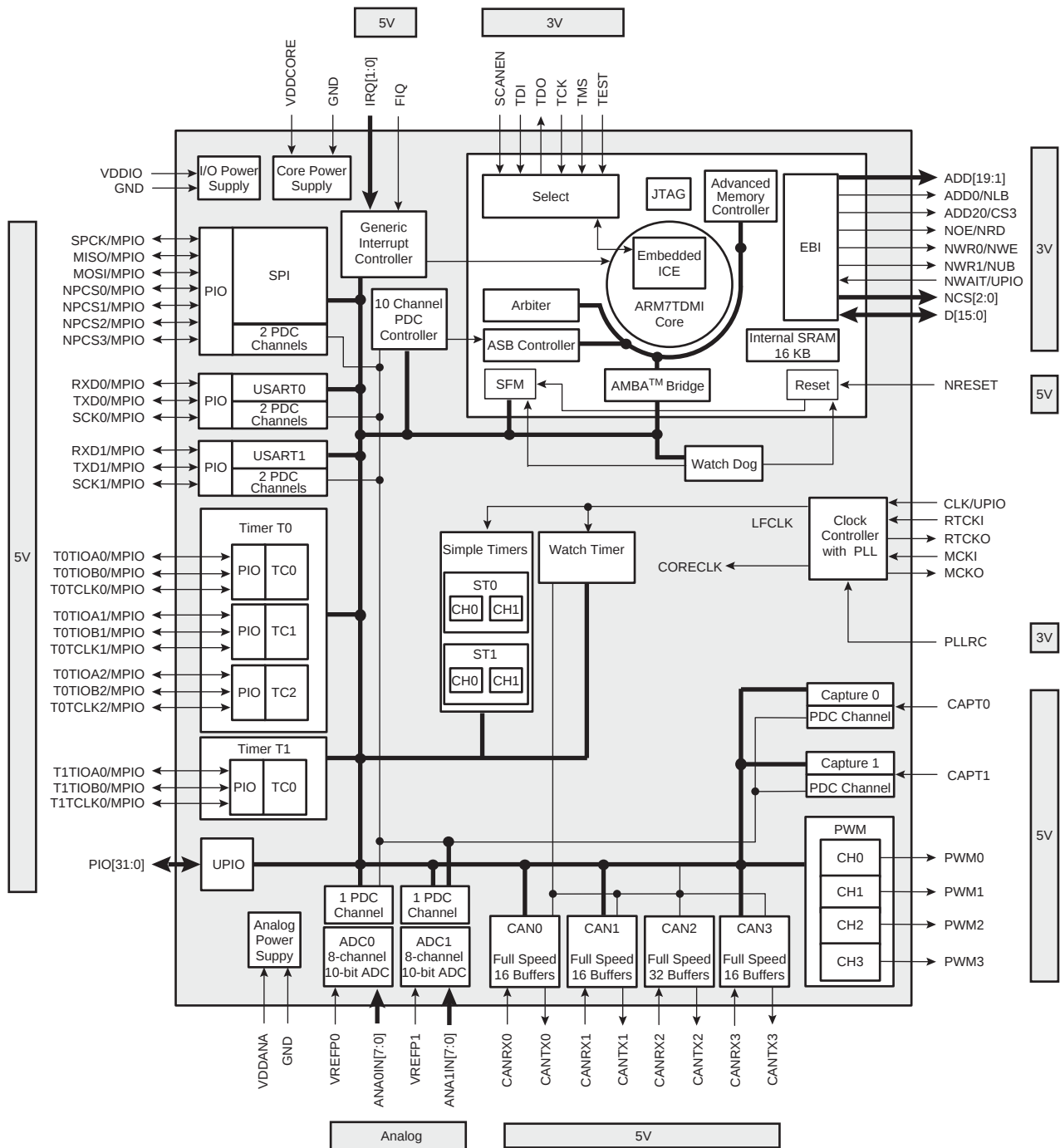
Figure 1. Block Diagram
