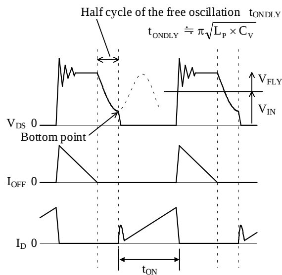
Figure 8-13. Ideal Bottom-on Operation Waveforms (Power MOSFET Turns On at the Lowest Voltage of V_{DS} Waveform)
