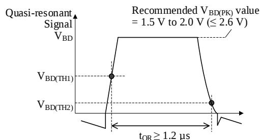
Figure 8-16. The Effective Pulse Width of Quasi-Resonant Signal
