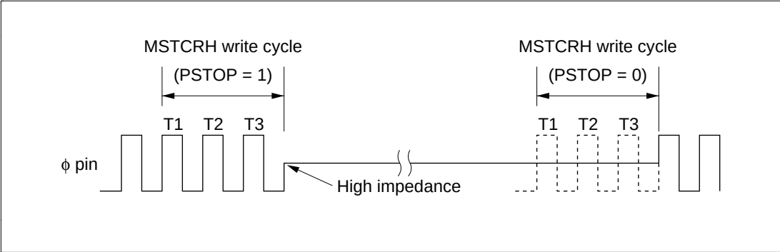
Figure 20.3 Starting and Stopping of System Clock Output
