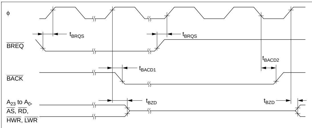
Figure 21.14 Bus-Release Mode Timing
