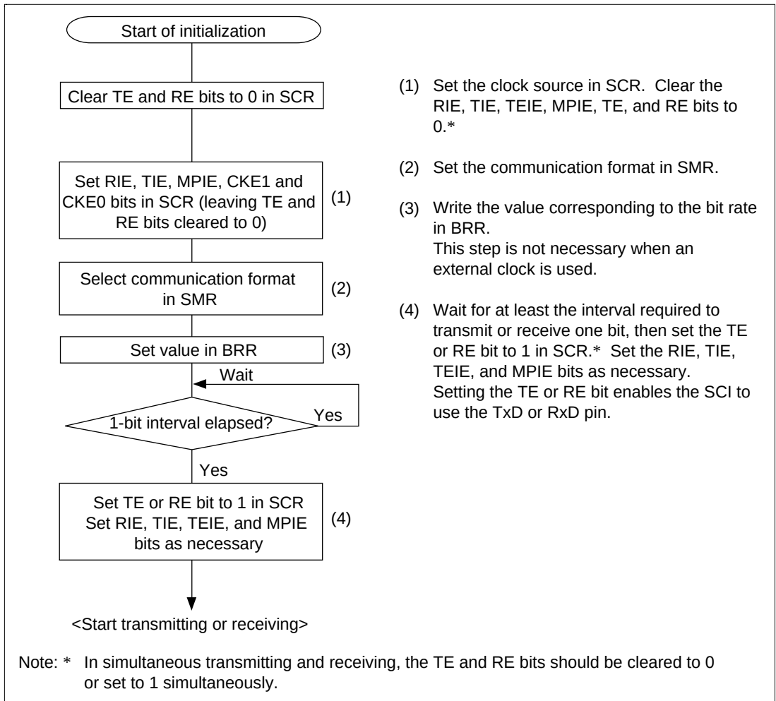
Figure 12.15 Sample Flowchart for SCI Initialization
