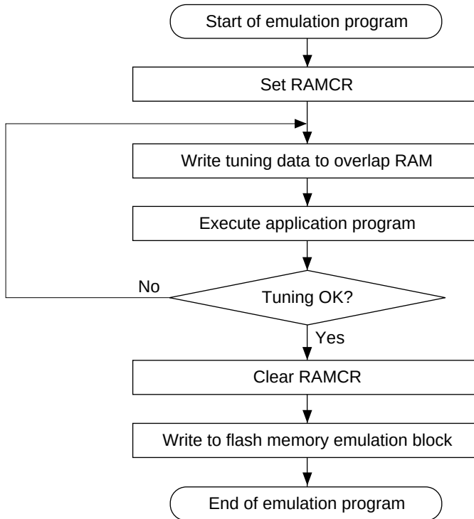
Figure 17.13 Flowchart of Flash Memory Emulation in RAM
