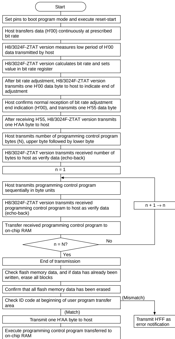
Figure 18.7 Boot Mode Execution Procedure
