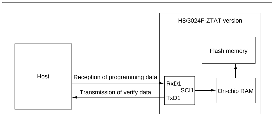
Figure 18.6 System Configuration When Using Boot Mode
