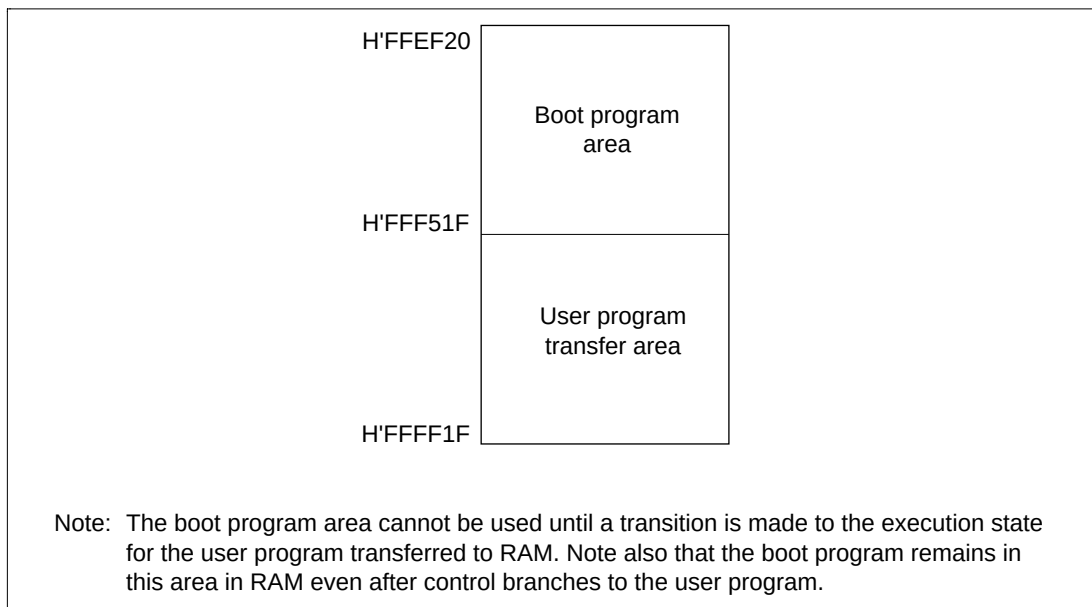
Figure 18.8 RAM Areas in Boot Mode
