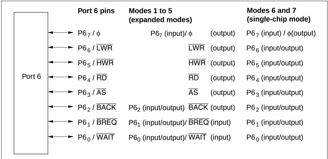
Figure 7.6 Port 6 Pin Configuration
