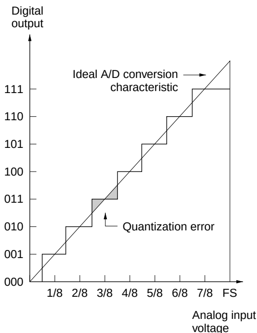
Figure 14.9 A/D Converter Accuracy Definitions (1)
