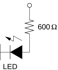
Figure 21.2 Sample LED Circuit
