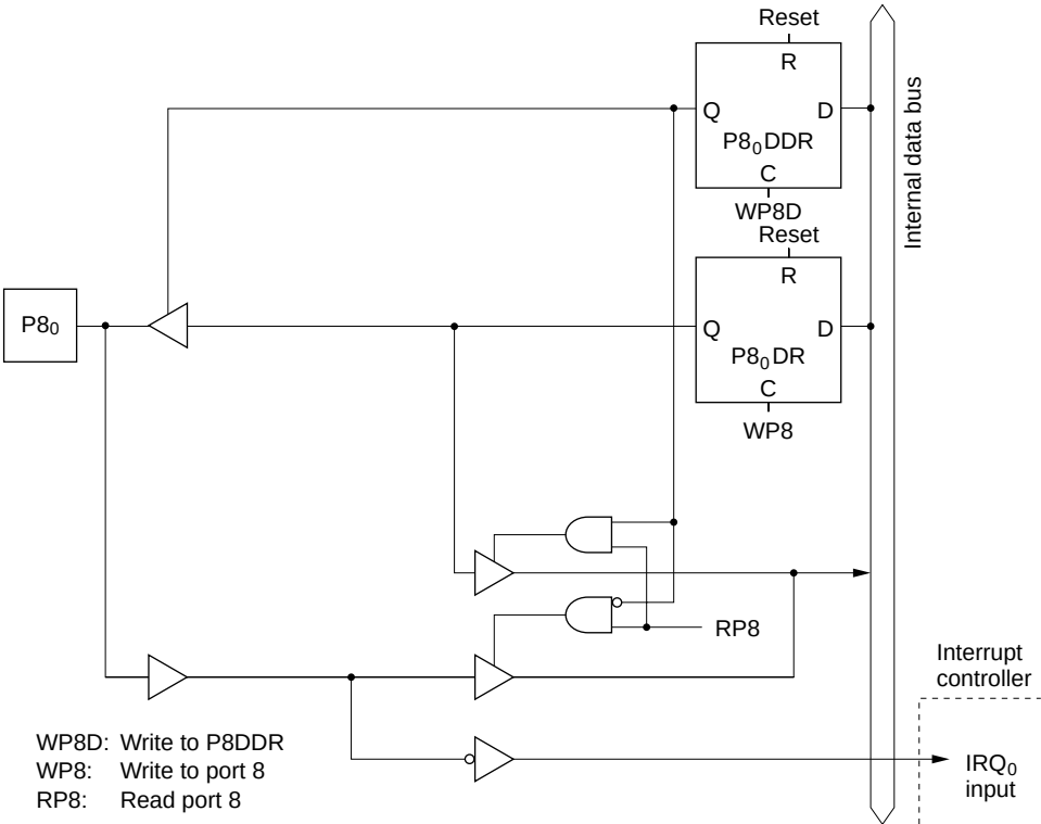
Figure C.8 (a) Port 8 Block Diagram (Pin P8 0 )
