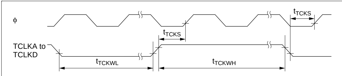
Figure 21.17 Timer External Clock Input Timing
