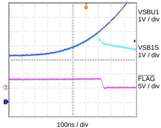
SBU OVP Transient
