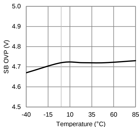
SB Switch OVP vs. Temperature
