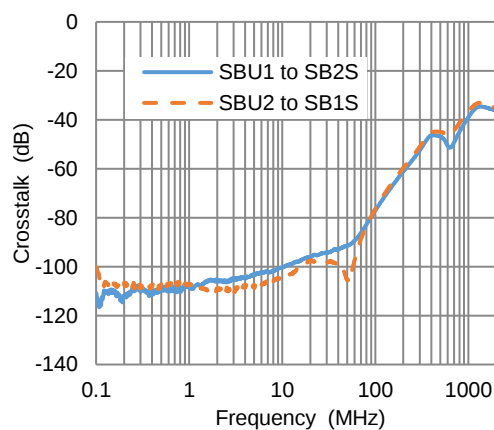
SBU Switch Crosstalk
