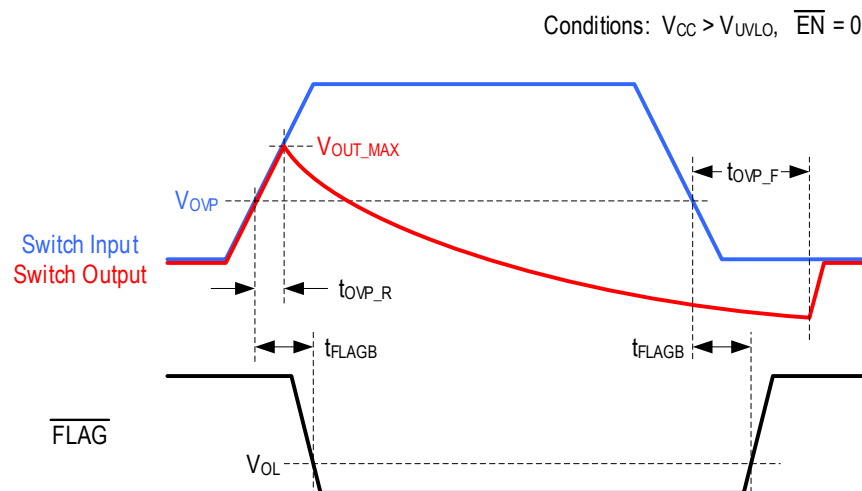
Figure 3. OVP Fault Protection Timing Diagram
