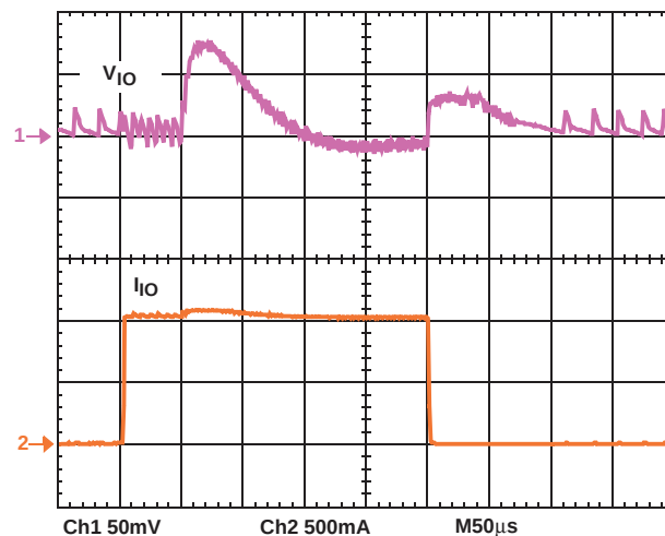
FIGURE 10. I/O CONVERTER LOAD TRANSIENT WITH MODE CHANGE
