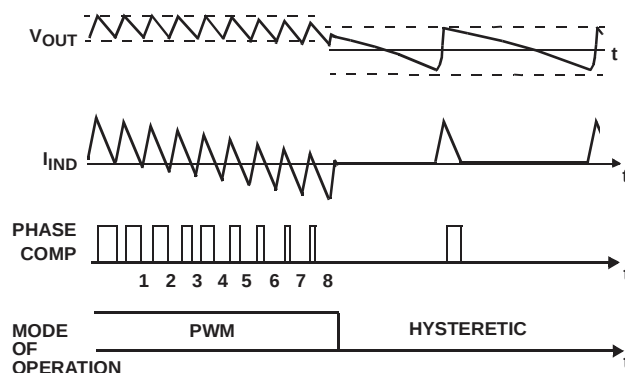
FIGURE 7. PWM TO HYSTERETIC TRANSITION
