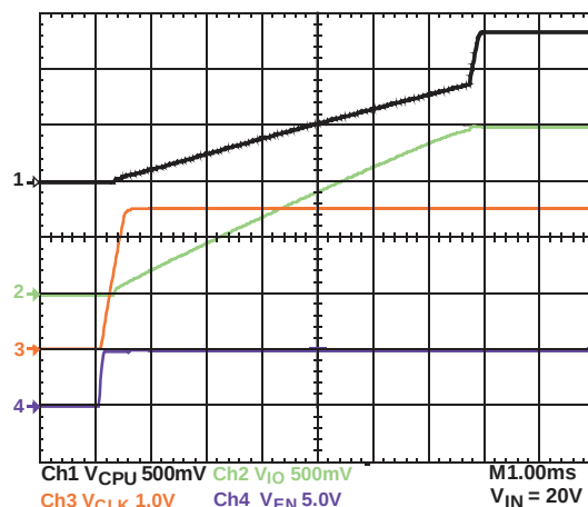
FIGURE 1. INITIAL STARTUP
