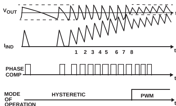
FIGURE 8. HYSTERETIC TO PWM TRANSITION
