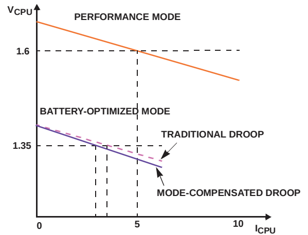
FIGURE 2. MODE-COMPENSATED DROOP
