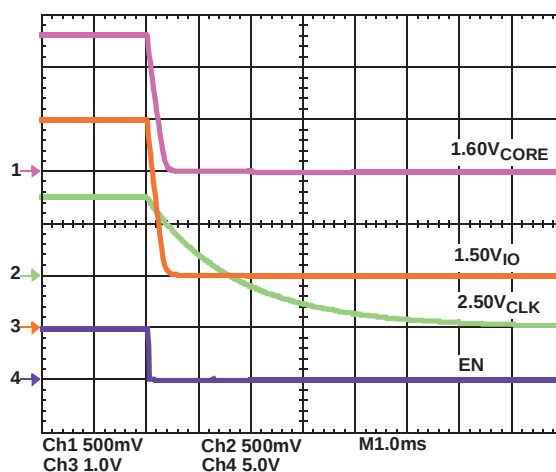
FIGURE 11. SHUTDOWN WAVEFORMS
