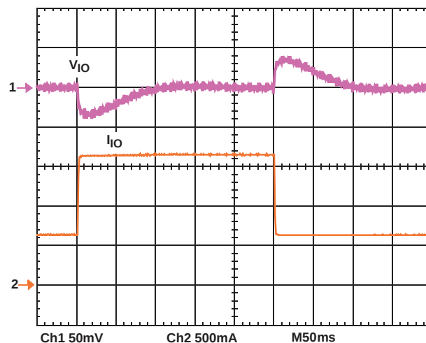
FIGURE 9. I/O CONVERTER LOAD TRANSIENT IN PWM MODE
