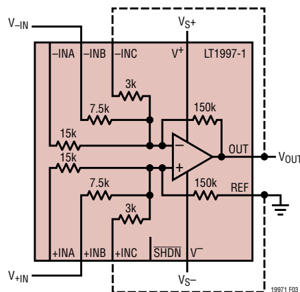
DIFFERENCE AMPLIFIER CONFIGURATION IMPLEMENTED WITH THE LT1997-1, R_F = 150\text{k} , R_G = 7.5\text{k} , GAIN = 20 ADDING THE DASHED CONNECTIONS CONNECT THE 3k RESISTOR IN PARALLEL WITH R_F , SO R_F IS REDUCED TO 2.94\text{k} . THE GAIN BECOMES 2.94\text{k}/7.5\text{k} = 0.392
