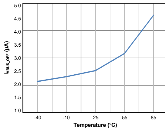
Figure 21. VBUS Shutdown Current vs. Temperature (VBUS=20V)
