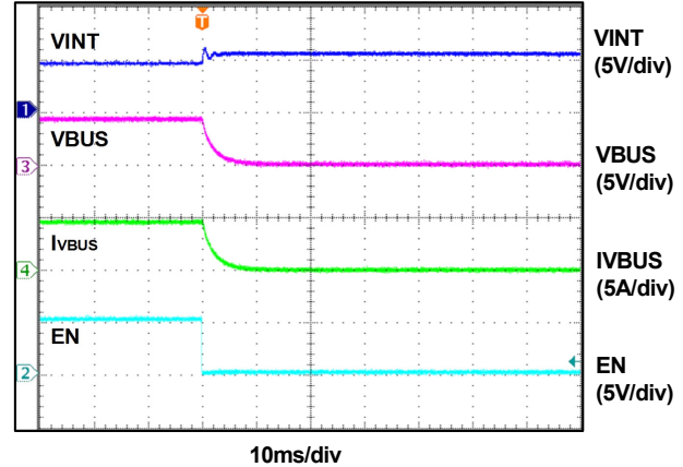
Figure 7. Turn-Off by EN (VINT = 5V)
