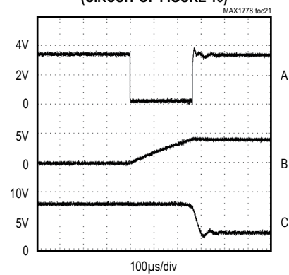
POWER-UP INTO SHORT-CIRCUIT (CIRCUIT OF FIGURE 10)
