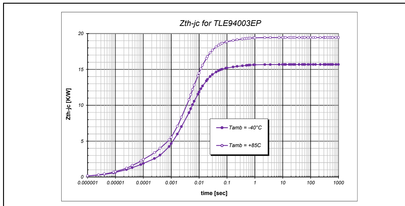
Figure 17 ZthJC Curve
