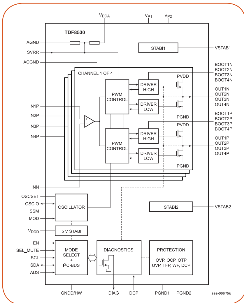
Block diagram
