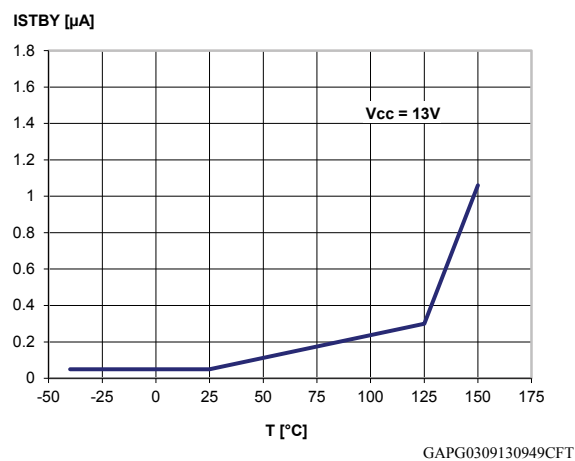
Figure 16. Standby current
