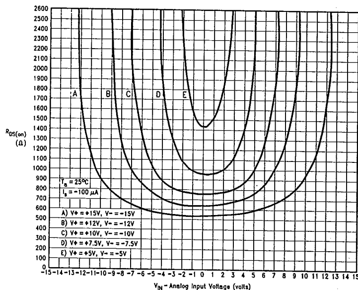
Figure 11: R_{DS(on)} vs Analog Signal Voltage
