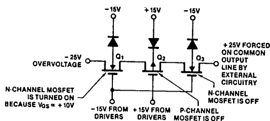
(b) OVERVOLTAGE WITH MUX POWER ON Figure 8: Overvoltage Protection
