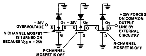
(a) OVERVOLTAGE WITH MUX POWER OFF
