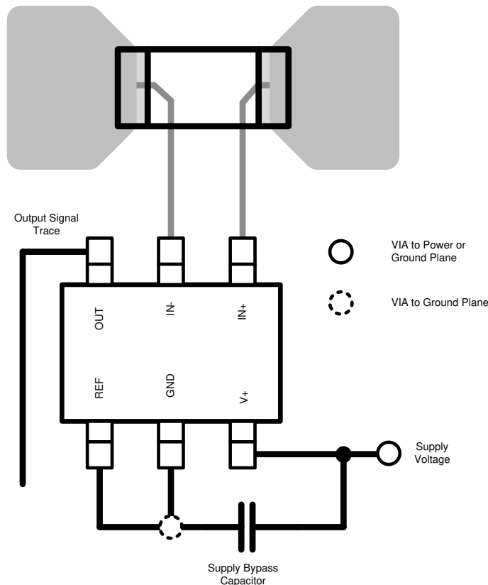
Figure 34. Recommended Layout
