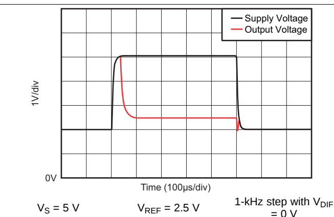
Figure 22. Brownout Recovery
