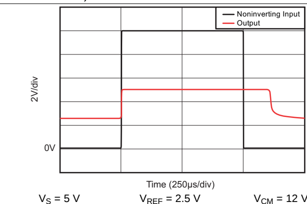
Figure 20. Noninverting Differential Input Overload
