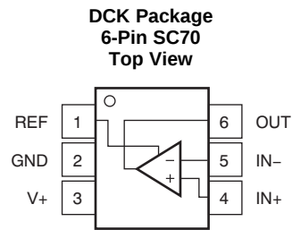
Pin Functions
