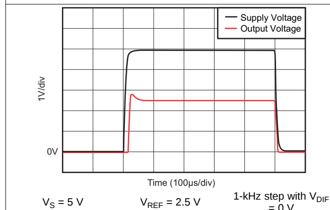
Figure 21. Start-Up Response
