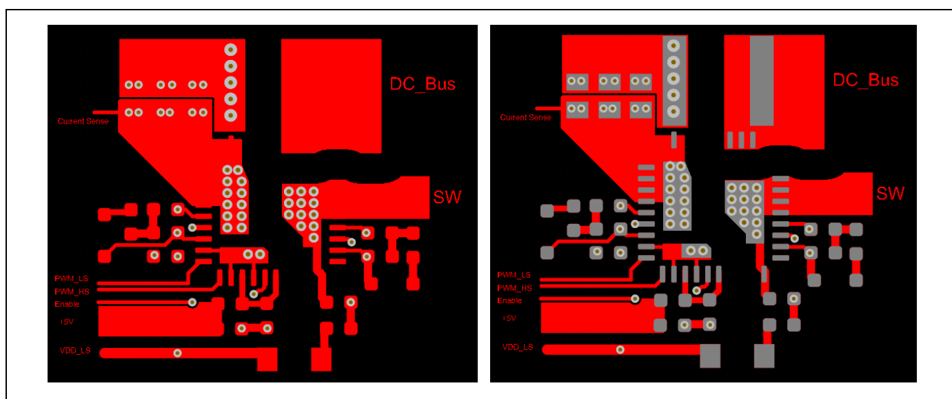
Figure 25 Top layer of the PCB (trace on the left and top solder paste layer on the right)
