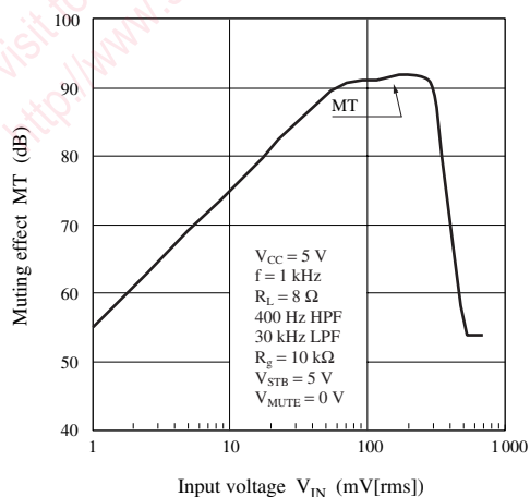
MT — V_{\text{IN}}
