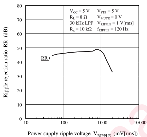
RR — V_{\text{RIPPLE}}
