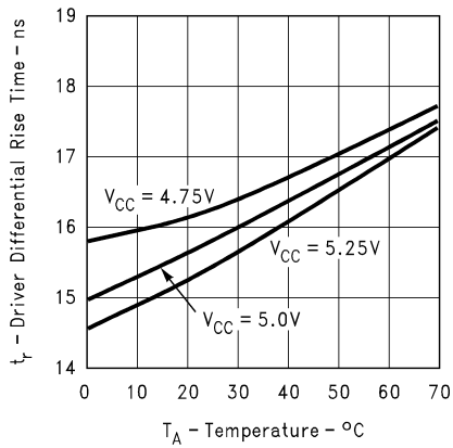
Driver Differential Rise Time vs V_{CC} vs Temperature
