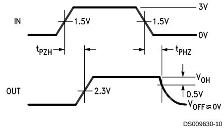
FIGURE 6. Driver Enable and Disable Times ( t_{PZH} , t_{PHZ} )
