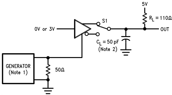
FIGURE 7. Driver Enable and Disable Times ( t_{PZL} , t_{PLZ} )
