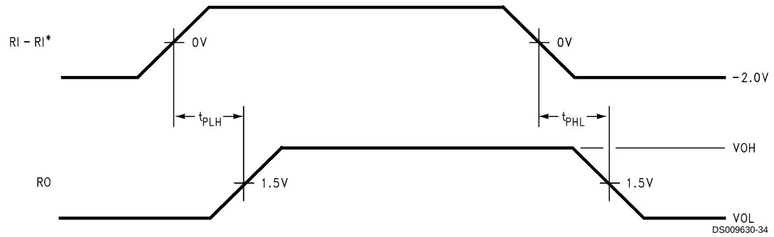
FIGURE 15. Typical Curve Receiver Propagation Delay Timing
