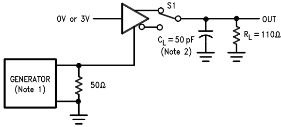
FIGURE 6. Driver Enable and Disable Times ( t_{PZH} , t_{PHZ} )
