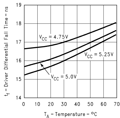
Driver Differential Fall Time vs V_{CC} vs Temperature
