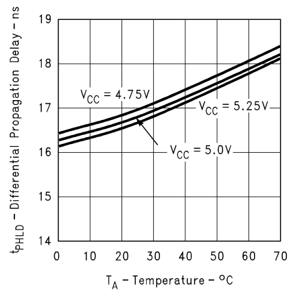
Driver Differential Propagation Delay vs V_{CC} vs Temperature
