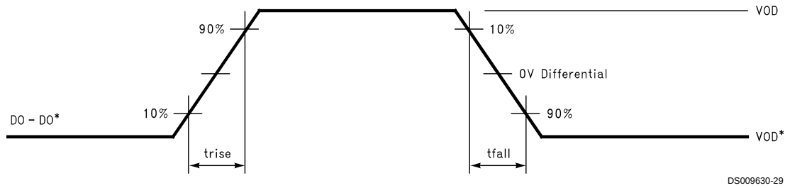
FIGURE 13. Typical Curve Driver Differential Rise and Fall Times
