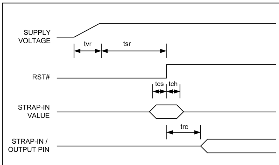
Figure 12. Reset Timing
