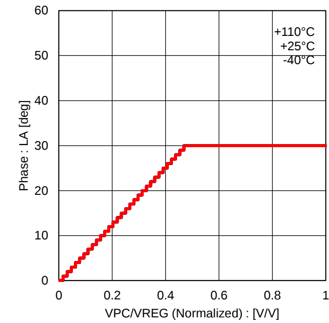
Figure 34. PC Voltage Normalized vs Lead Angle
