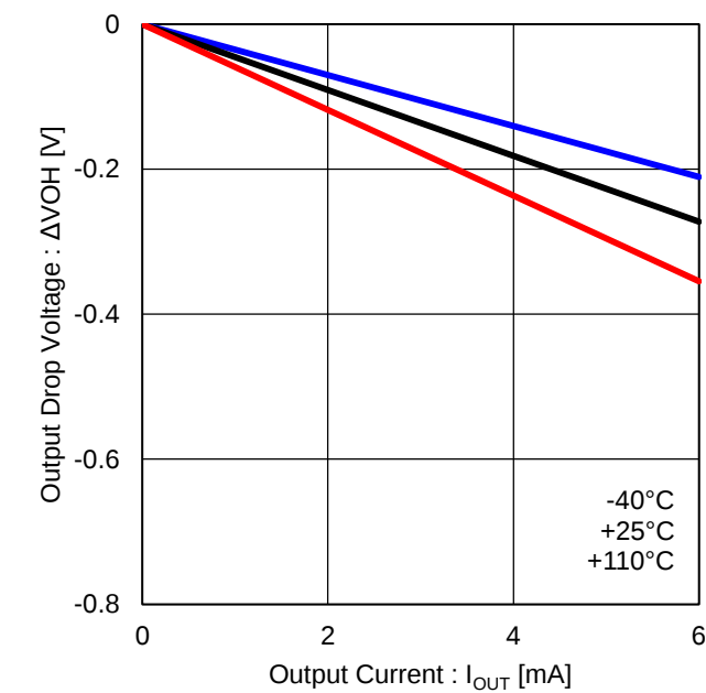
Figure 36. High Side Output Voltage (FG)
