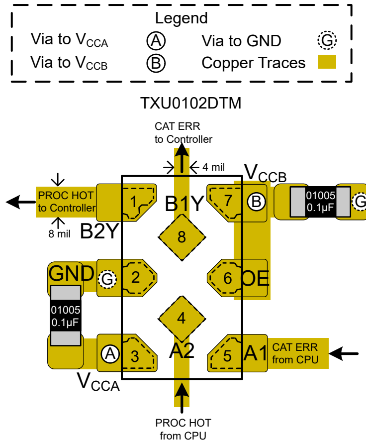
Figure 12-1. Layout Example – TXU0102
