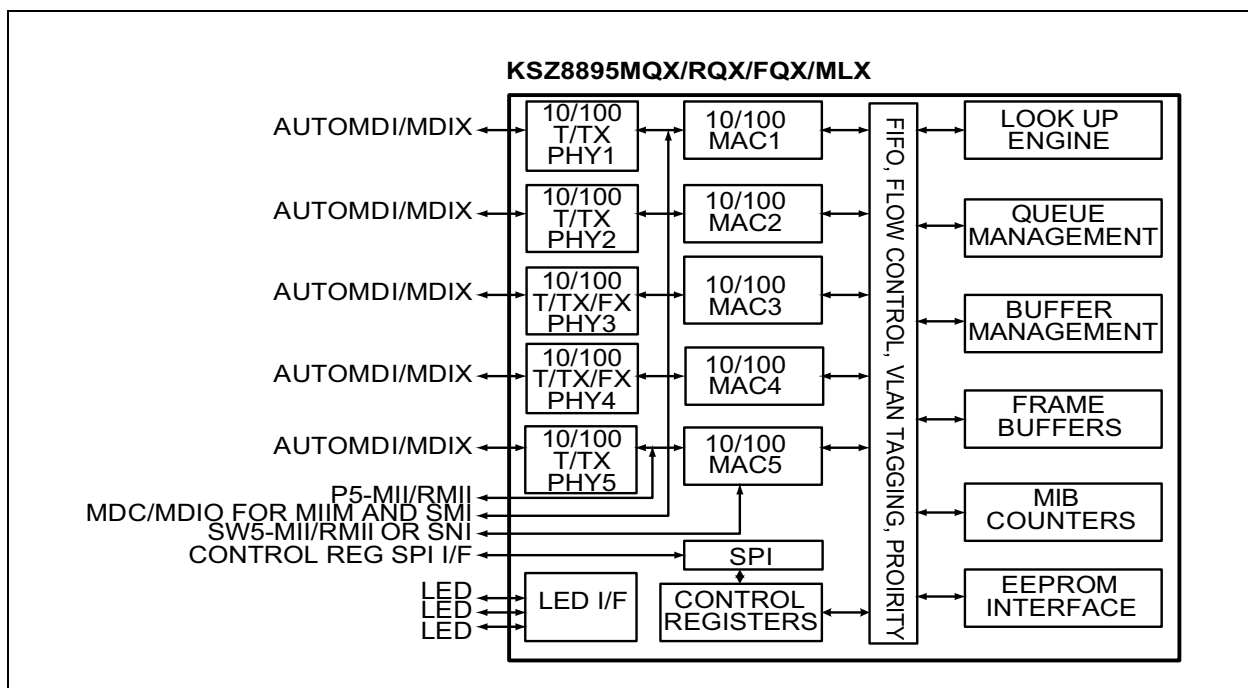
FIGURE 1-1: FUNCTIONAL DIAGRAM
