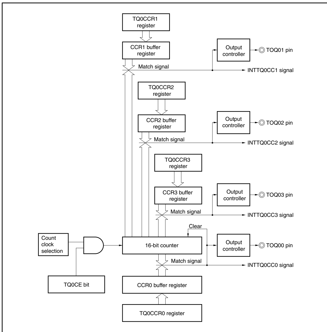
Figure 8-6. Configuration of TQ0CCR1 to TQ0CCR3 Registers
