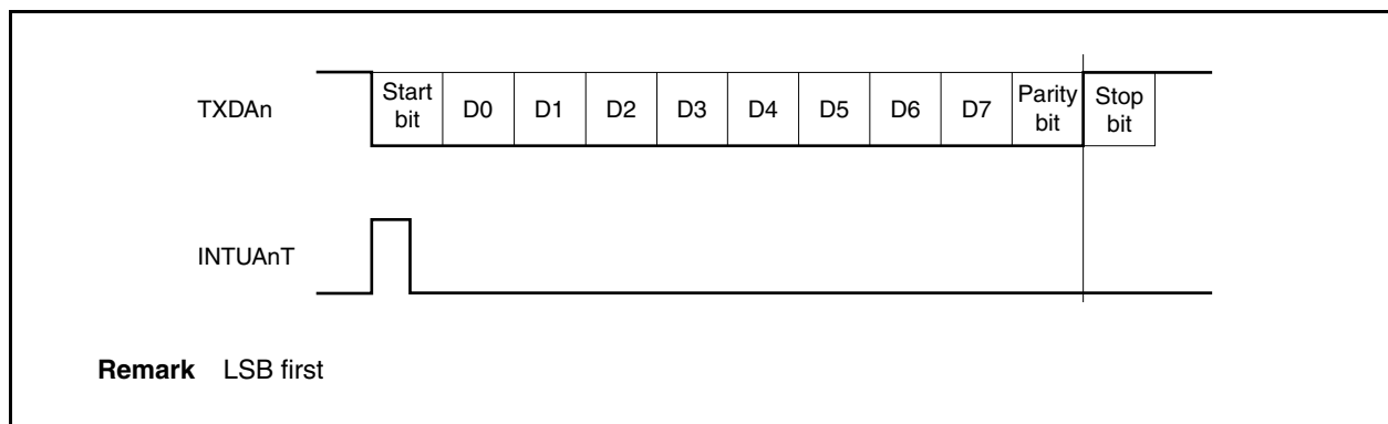
Figure 15-10. UART Transmission
