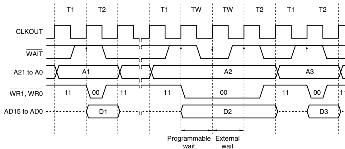
Figure 5-11. Separate Bus Write Timing (Bus Size: 16 Bits, 16-Bit Access)
