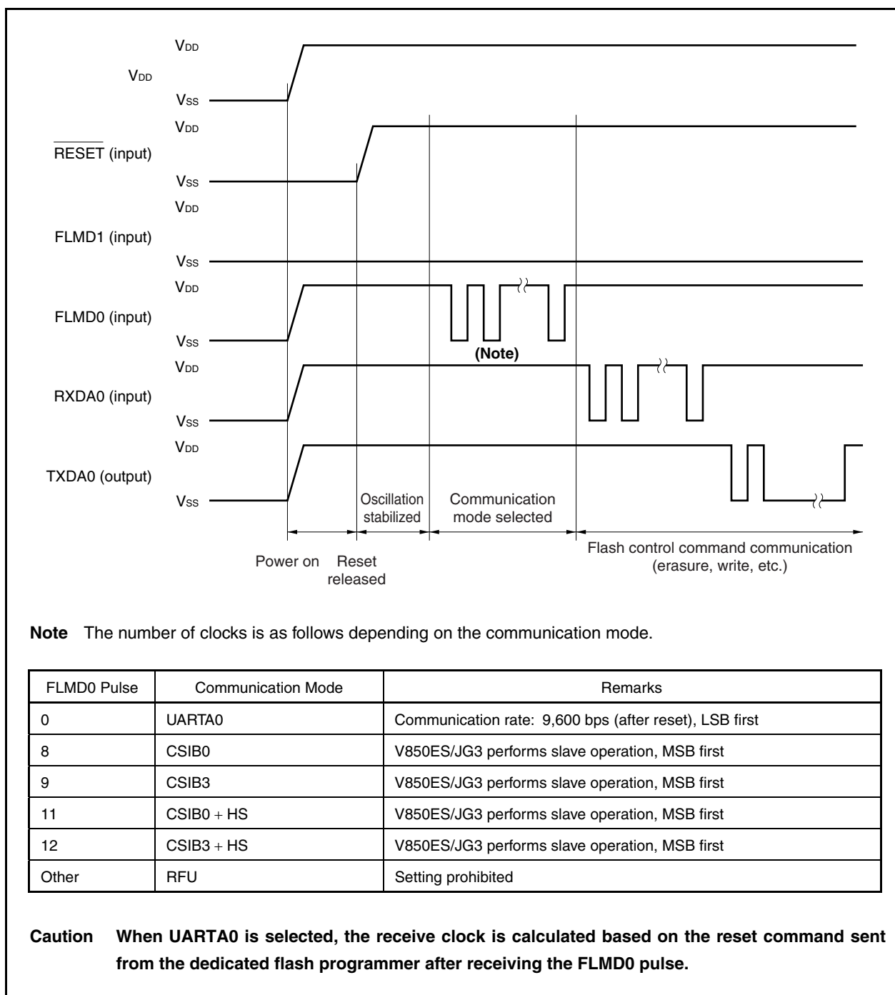
Figure 27-8. Selection of Communication Mode
