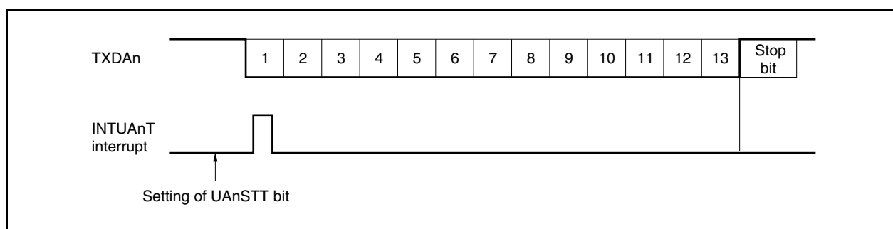
Figure 15-8. SBF Transmission
