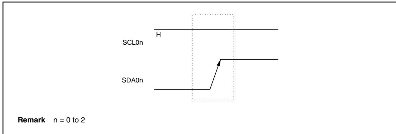
Figure 17-12. Stop Condition
