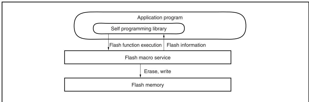
Figure 27-15. Concept of Self Programming
