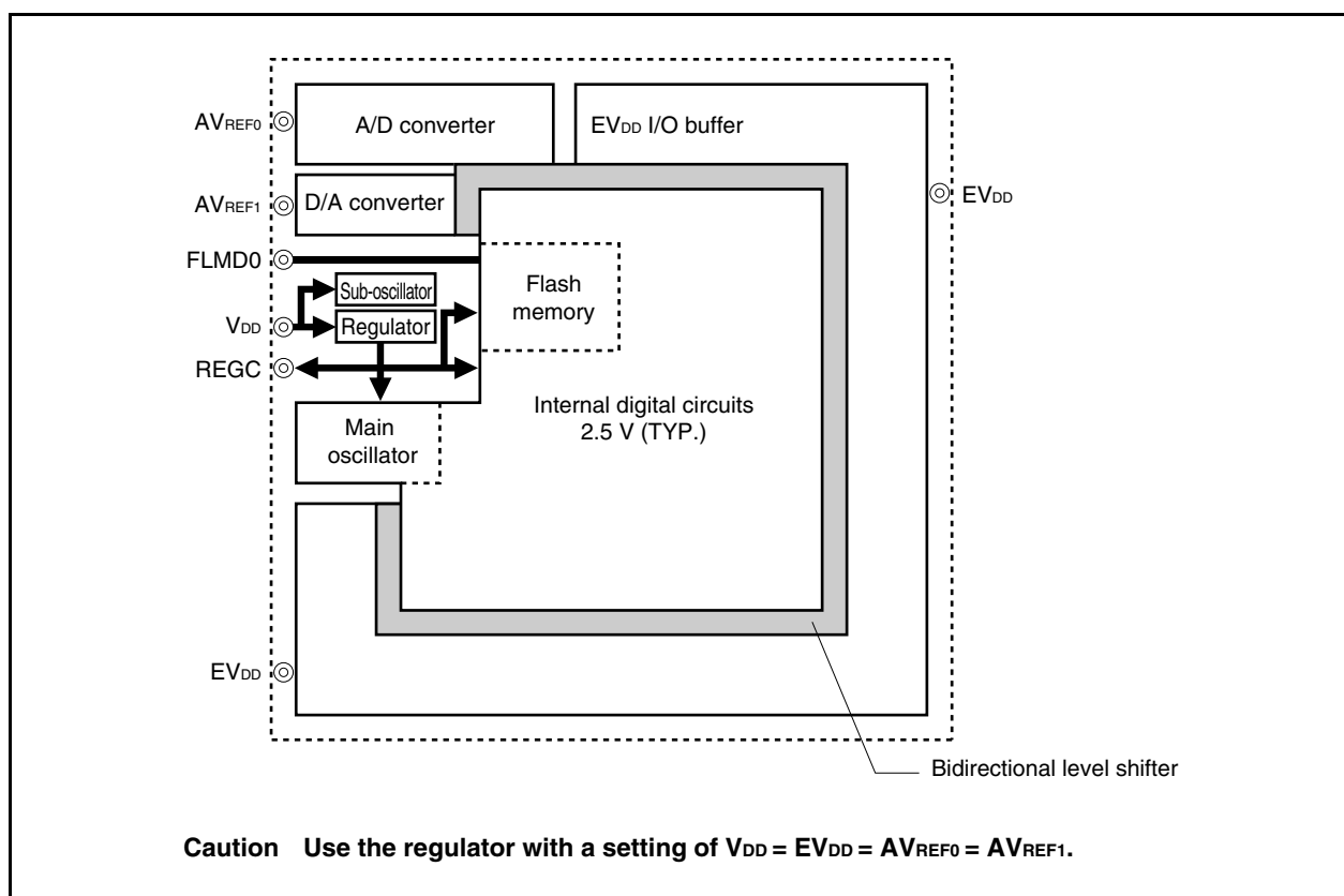
Figure 26-1. Regulator
