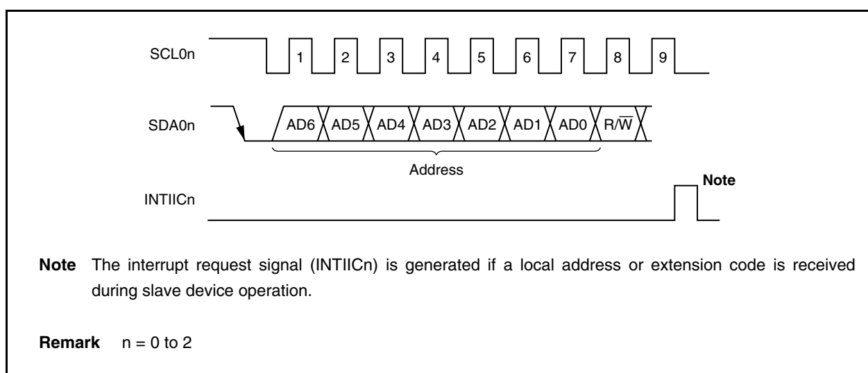
Figure 17-9. Address
