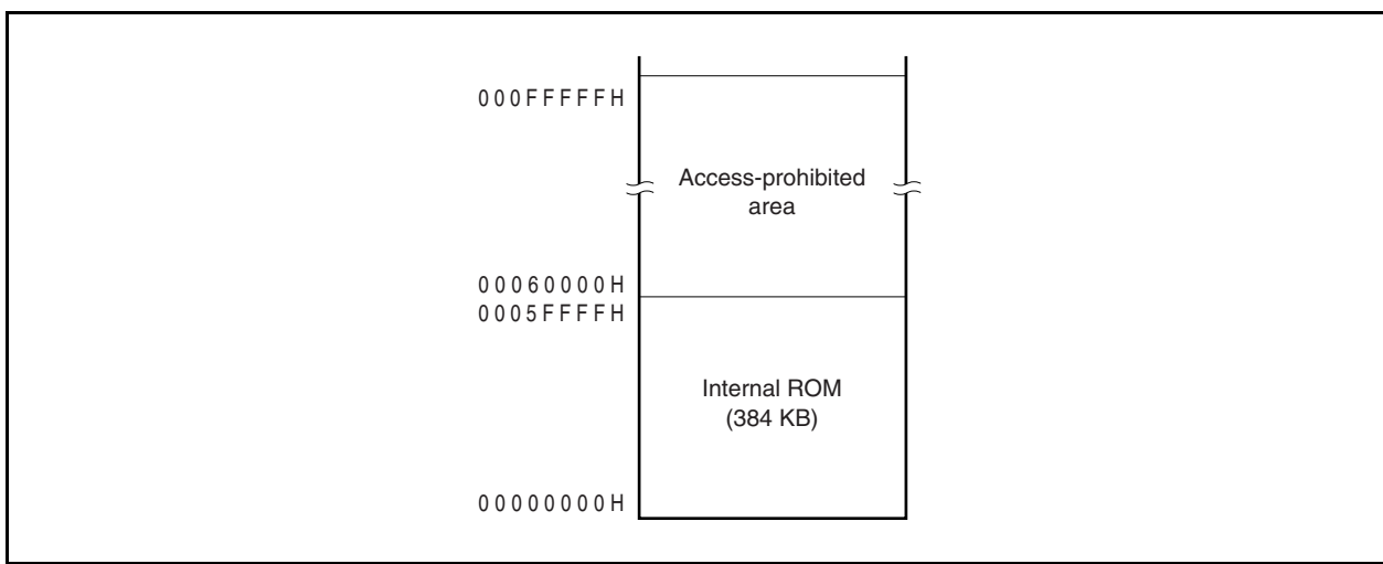
Figure 3-4. Internal ROM Area (384 KB)
