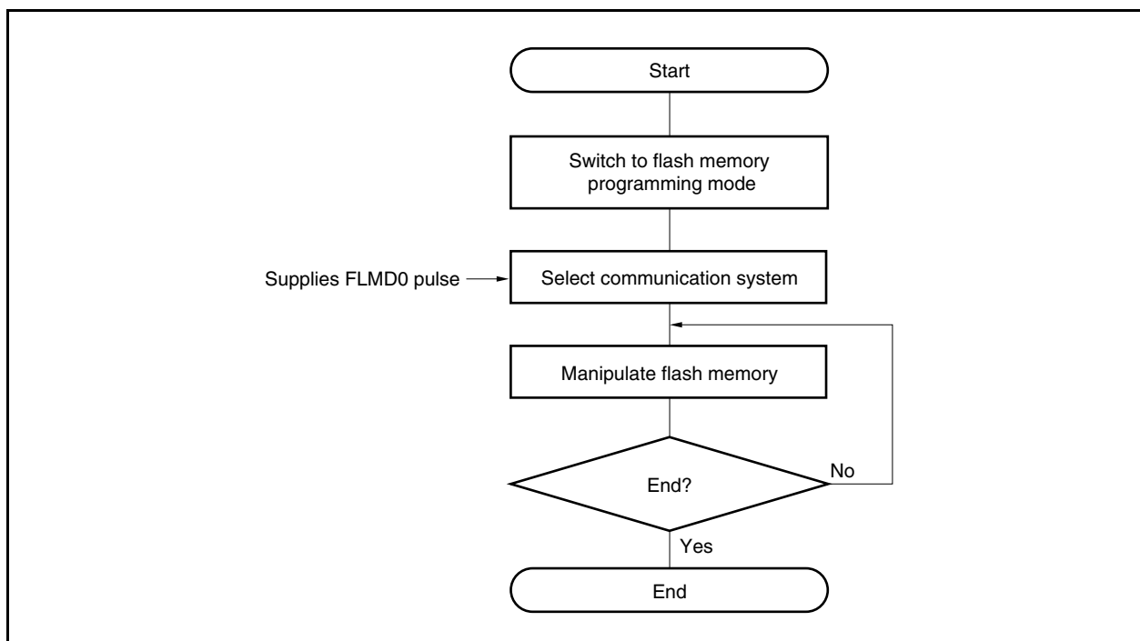
Figure 27-7. Procedure for Manipulating Flash Memory
