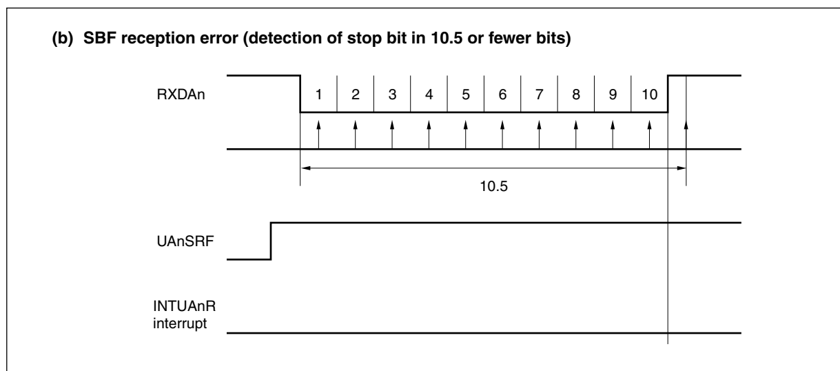
Figure 15-9. SBF Reception (2/2)
