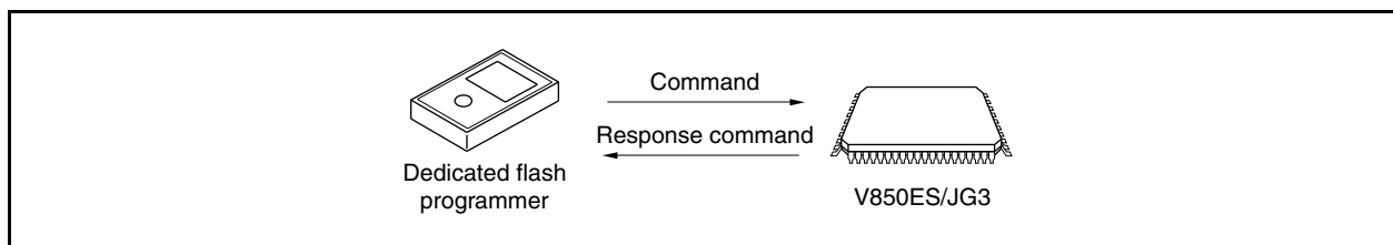
Figure 27-9. Communication Commands
