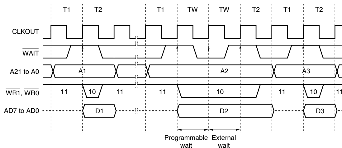
Figure 5-12. Separate Bus Write Timing (Bus Size: 8 Bits)
