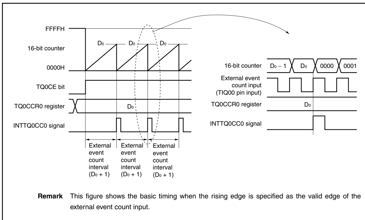
Figure 8-10. Basic Timing in External Event Count Mode
