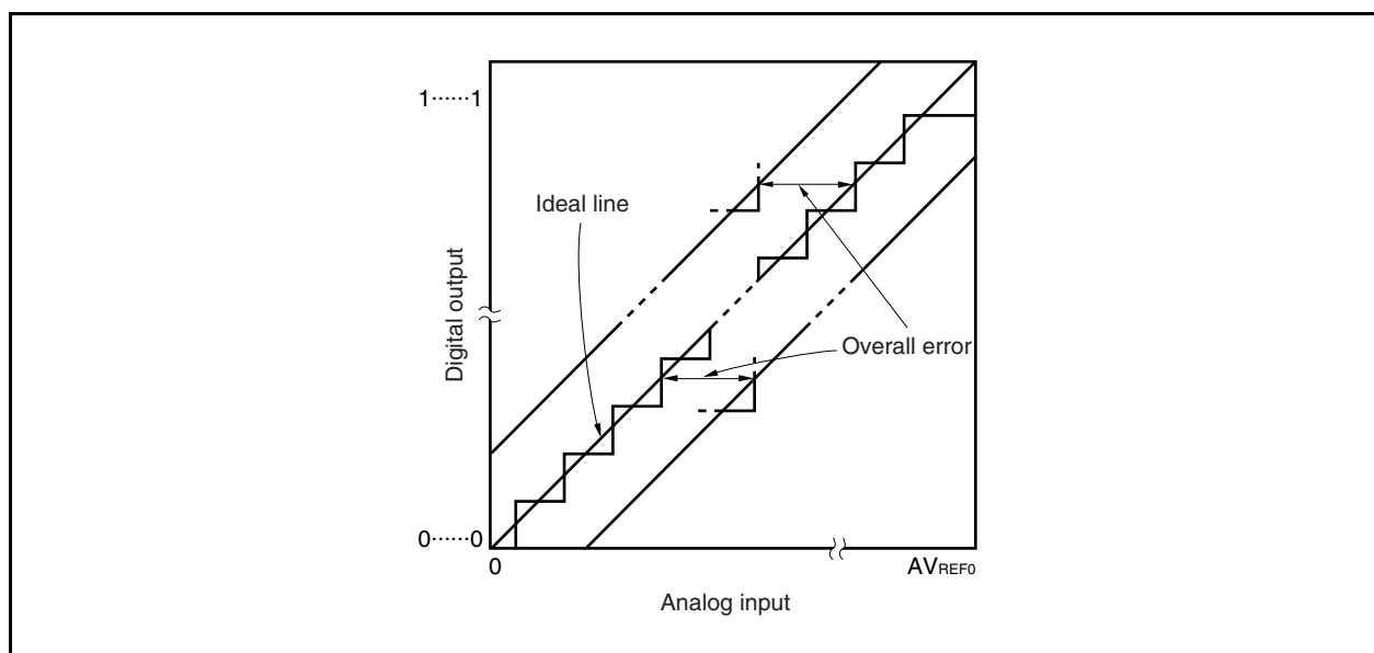
Figure 13-16. Overall Error
