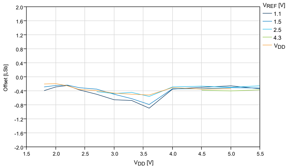
Figure 37-48. Offset Error vs. V_{DD} ( f_{ADC} = 115 kps) at T = 25^{\circ}C , REFSEL = Internal Reference
