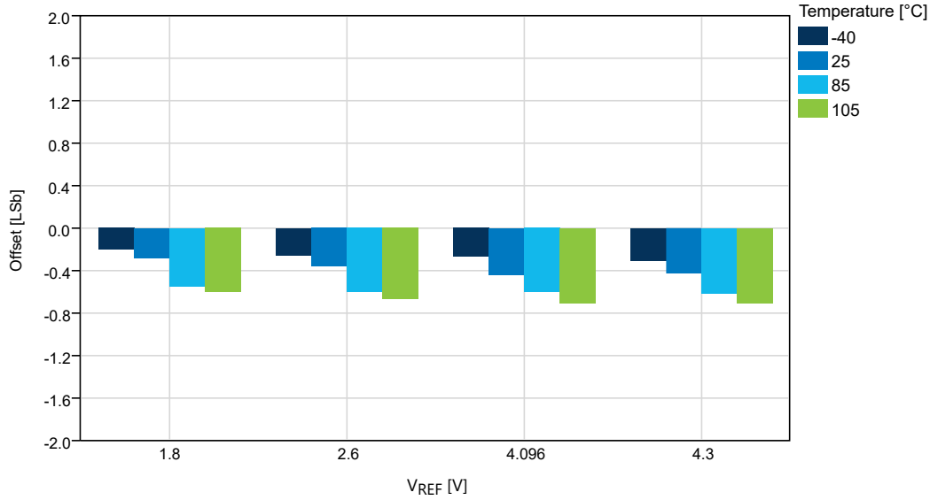
Figure 37-59. Offset vs. V_{REF} ( V_{DD} = 5.0V , f_{ADC} = 115 kps, REFSEL = \text{External Reference} )
