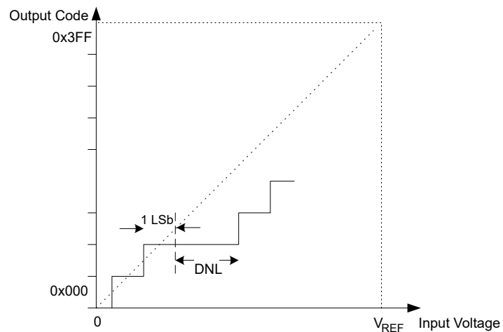
Figure 35-4. Differential Nonlinearity
