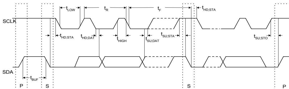
Figure 9.2 SMBus Timing
