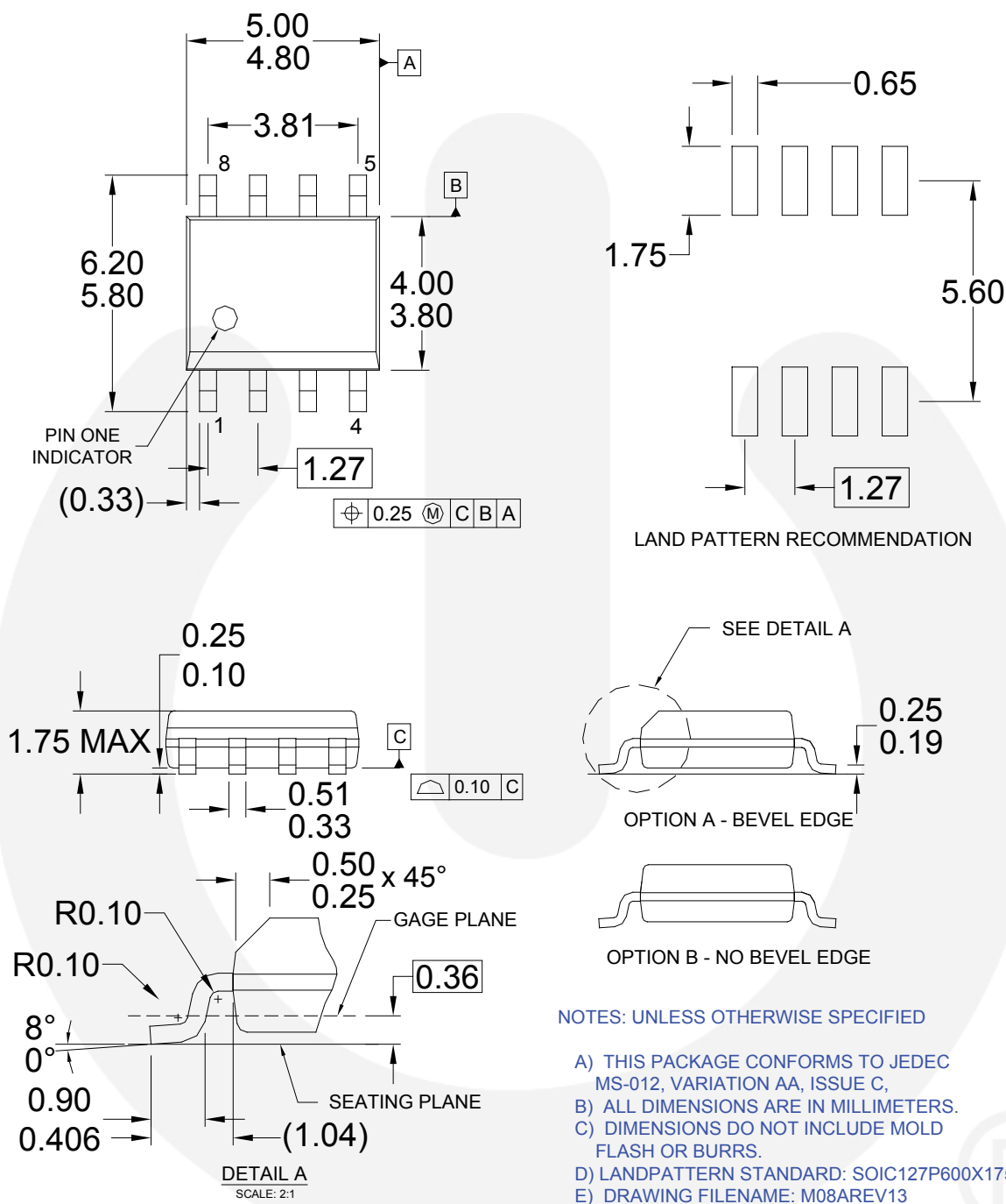
Figure 18. SOIC-8 Package
